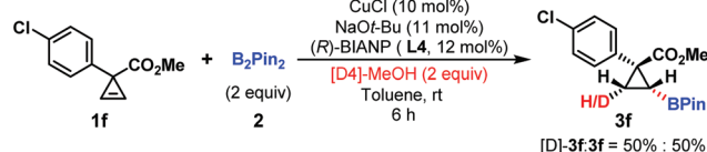
Scheme 4 [D4]-Methanol experiment.
