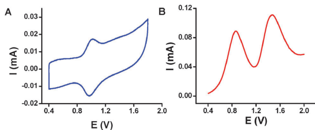
Fig. 2 (A) Representative cyclic voltammogram (CV) of the replicated 2 -based TL' formed by disassembly of 2 - and 3 -based SPMA with \text{PET}_3 and selective transfer of osmium complex 2 to ITO substrates functionalized with CLs. The scan rate is 400 \text{ mV s}^{-1} . (B) Differential pulse voltammogram (DPV) of the reaction solution after the disassembly of 2 - and 3 -based SPMA with \text{PET}_3 . The following conditions were applied: scan rate: 20 \text{ mV s}^{-1} , pulse width: 16 ms, pulse amplitude: 50 mV, and pulse period, 200 ms. For both (A) and (B) electrolyte: 0.1 \text{ M TBABF}_4/\text{CH}_3\text{CN} was used at room temperature. Pt wire and \text{Ag}/\text{AgCl} were used as counter and reference electrodes, respectively. The functionalized ITO-coated glass substrates were used as working electrodes.
