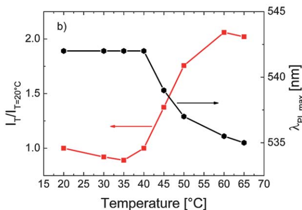
Fig. 3 (a) The effect of temperature on the fluorescence characteristics of P-2 in PBS (0.1 g L -1 ). The excitation wavelength was 435 nm. (b) The correlation between \lambda_{\text{PL,max}}^{\text{PL}} , the relative emission intensity ( I_T/I_{T=20^\circ\text{C}} ), and the temperature of the solution. Data are taken from the spectra in (a).
