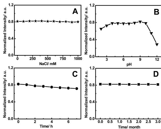
Fig. 4 (A) The relative fluorescence intensity at 427\text{ nm} (excitation at 344\text{ nm} ) of the FNCsPs in the NaCl solution. (B) Dependence of the fluorescence intensity on the pH values from 2 to 12. (C) The variation of the fluorescence intensity of the FNCsPs under irradiation by a 500\text{ W} Xe lamp for different time intervals. (D) Photostability of the FNCsPs as a function of the storage time.
