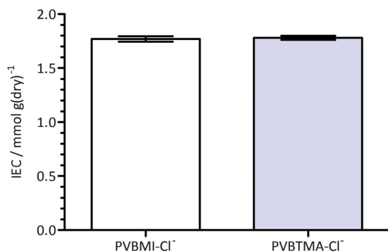
Fig. 3 The ion-exchange capacities (IEC) of the chloride-form benzylmethylimidazolium ( PVBMI-Cl - ) and benzyltrimethylammonium ( PVBtMA-Cl - ) radiation-grafted anion-exchange membranes. Error bars are confidence intervals at the 95% confidence level.
