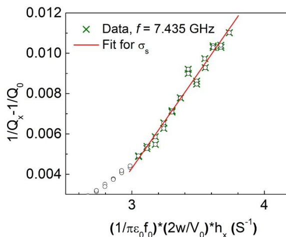
Fig. 3. Plot of cavity perturbation data ( 1/Q_x - 1/Q_0 ) as a function of the normalized specimen area ( w \times h_x ) for graphene inks at the resonant frequency of 7.435 \text{ GHz} . Q_0 is the quality factor of the empty cavity, and Q_s is the quality factor of the cavity loaded with the specimen. 33 Symbols represent experimental data, and the solid line represents a linear fit to the cavity perturbation equation through the data points. In the presented notation, the microwave surface conductivity is obtained directly from the slope of the linear portion of the cavity perturbation plot, \sigma_s = (9.3 \times 10^{-3} \pm 3 \times 10^{-4}) \text{ S} .
