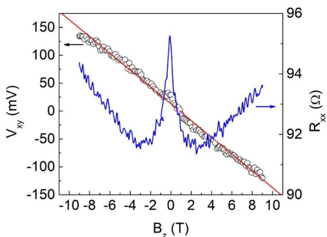
Fig. 2. Hall voltage ( V_{xy} , open circles) as a function of magnetic field ( B_z ) at I_x of 1.0 \mu\text{A} and temperature of 5 \text{ K} . The straight line represents a linear fit through the data points. The negative slope indicates that the majority charge carriers are holes. A characteristic peak in the plot of R_{xx} versus B_z is consistent with 2D charge transport, as discussed later.
