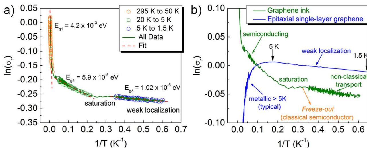
Fig. 4. (a) Logarithm of relative conductivity ( \sigma_r = 1/(R_{xx}/R_0) ) versus reciprocal temperature ( 1/T ) referenced to R_{xx} at 273 K. (b) Comparison of the temperature-dependent conductivity of the percolating network generated from cellulose-stabilized graphene inks (green line) with that of epitaxial graphene with a carrier density of \approx 2 \times 10^{11} \text{ cm}^{-2} (blue line) referenced for clarity to R_{xx} at 10 K.
