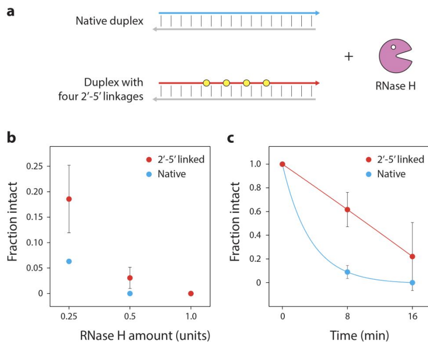
Figure 4. Testing ribonuclease activity on 2'-5'-linked structures. (a) Native and modified duplexes with four 2'-5' linkages were tested for resistance against RNase H. (b) Percent structure intact after 16-min incubation with different amounts of RNase H. (c) Digestion trend of native and modified duplexes with 0.5 units RNase H.
