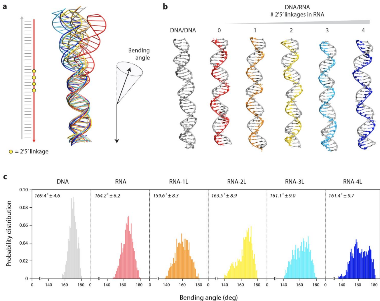
Figure 3. Molecular dynamics simulations of 2'-5'-linked DNA/RNA hybrid duplexes. (a) Superposition of centroids of all the structures analyzed. (b) Simulated structures of each variation, with the DNA strand shown in grey (constant in all the structures). RNA strands with none to four 2'-5' linkages are shown in different colors for clarity. (c) Interhelical bending angle distribution of the simulated structures, color coded as in (b). 1L to 4L = one to four 2'-5' linkages.
