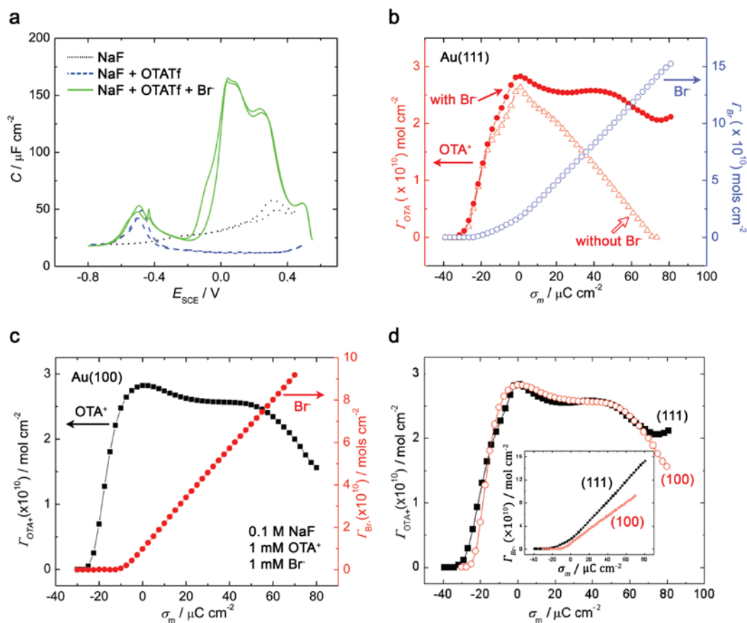
Fig. 2. (a) Differential capacity curves for Au(111) in 0.10 M NaF electrolyte (black dotted) and 1.0 mM OTATf in the absence and presence of 0.1 mM NaBr. (b) Surface excesses versus electrode charge density at the Au(111)/0.1 M NaF interface for 1.0 mM \text{OTA}^+ in the absence and presence of 1.0 mM NaBr and for 1.0 mM \text{Br}^- in the presence of 1.0 mM OTATf. (c) Surface excesses versus electrode charge density at the Au(100)/0.1 M NaF interface for 1.0 mM \text{OTA}^+ in the presence of 1.0 mM NaBr and 1.0 mM \text{Br}^- in the presence of 1.0 mM OTATf. (d) Overlaid Au(111) and Au(100) adsorption isotherms for 1.0 mM \text{OTA}^+ in the presence of 1.0 mM NaBr; (inset) corresponding adsorption isotherms for 1.0 mM \text{Br}^- in the presence of 1.0 mM OTATf. (a) and (b) are reproduced with permission from ref. 70. Copyright 2012 American Chemical Society. (c) and (d) are reproduced with permission from ref. 71. Copyright 2012 American Chemical Society.
