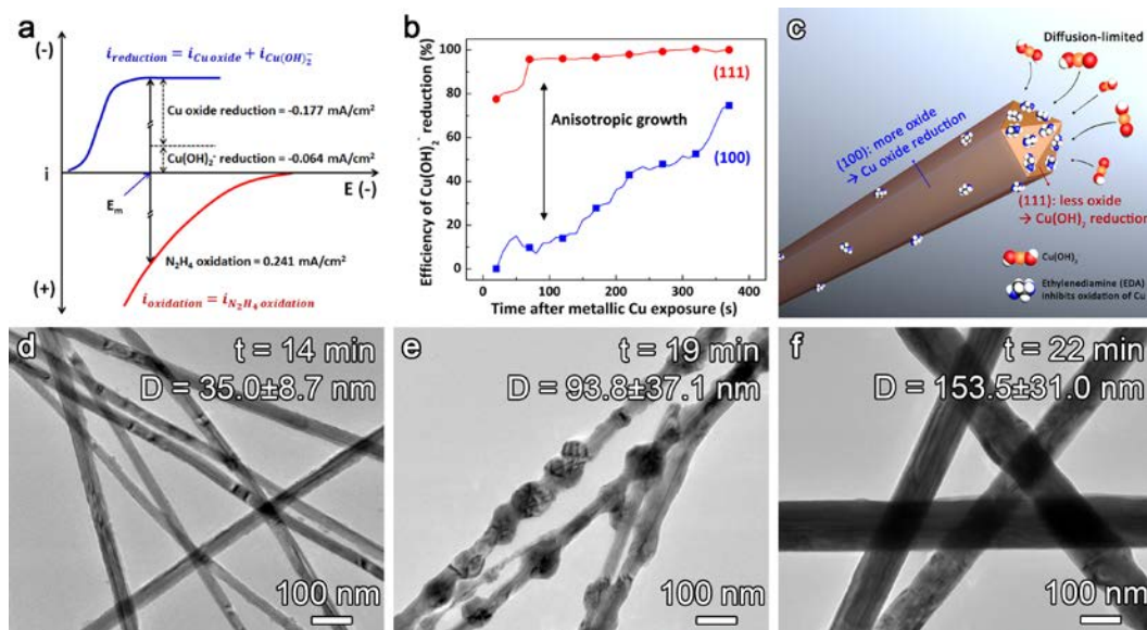
Fig. 7. (a) A diagram for mixed potential theory for EDA-based Cu nanowire growth. (b) Faradaic efficiency of \text{Cu(OH)}_2^- reduction to \text{Cu}^0 on Cu(111) and Cu(100) single-crystal electrodes. (c) Growth mechanism of Cu nanowires in the presence of EDA and NaOH. TEM images of Cu nanowires at (d) 14 min, (e) 19 min, and (f) 22 min after starting the reaction. (a)–(c) are reproduced with permission from ref. 42. Copyright 2017 American Chemical Society. (d)–(f) are reproduced with permission from ref. 30. Copyright 2014 Royal Society of Chemistry.
