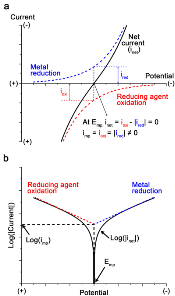
Fig. 4. (a) A diagram for mixed potential theory and (b) corresponding Tafel plot to obtain the current at the mixed potential. Reproduced with permission from ref. 43. Copyright 2018 American Chemical Society.
