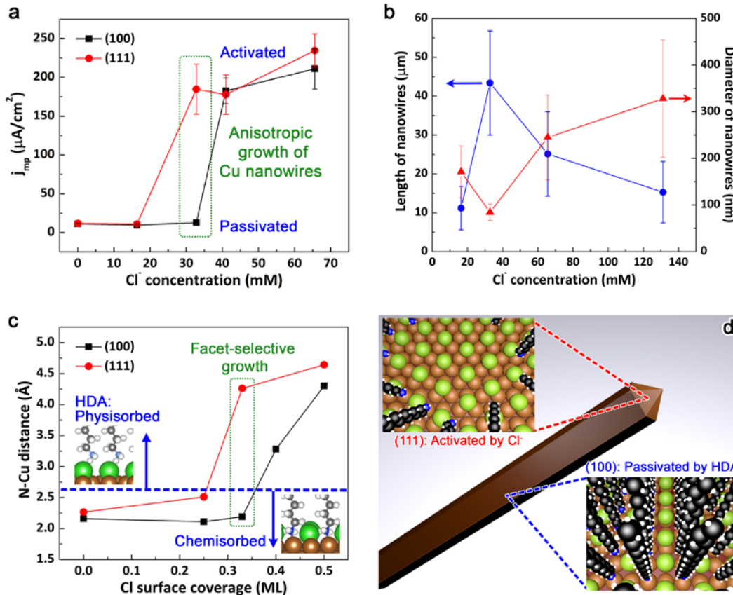
Fig. 6. (a) The current density at E_{mp} as a function of Cl^- concentration. (b) The average length and diameter of Cu nanowires synthesized with varying Cl^- concentrations. (c) N-Cu distance according to Cl surface coverage for Cu(100) and (111) surfaces. (d) A schematic for the growth of Cu nanowires in the presence of Cl^- and HDA showing {111} facets at the ends of nanowires activated by Cl^- for atomic addition and {100} facets on the sides completely passivated by the SAM of HDA. Reproduced with permission from ref. 43. Copyright 2018 American Chemical Society.
