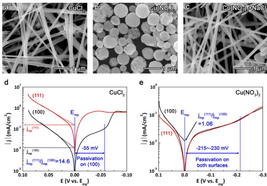
Fig. 5. Cu nanocrystals synthesized from (a) \text{CuCl}_2 , (b) \text{Cu}(\text{NO}_3)_2 , and (c) \text{Cu}(\text{NO}_3)_2 and \text{NaCl} , all in the presence of HDA and ascorbic acid. Tafel plots collected on Cu(111) and Cu(100) single-crystal electrodes in the electrolytes of (d) \text{CuCl}_2 and (e) \text{Cu}(\text{NO}_3)_2 with HDA and ascorbic acid. Reproduced with permission from ref. 43. Copyright 2018 American Chemical Society.
