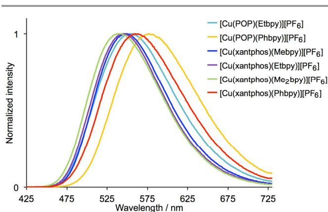
Fig. 8. Normalized emission spectra of solid [Cu(P ^A P)(N ^A N)][PF 6 ]. For \lambda_{exc} , see Table 1.
