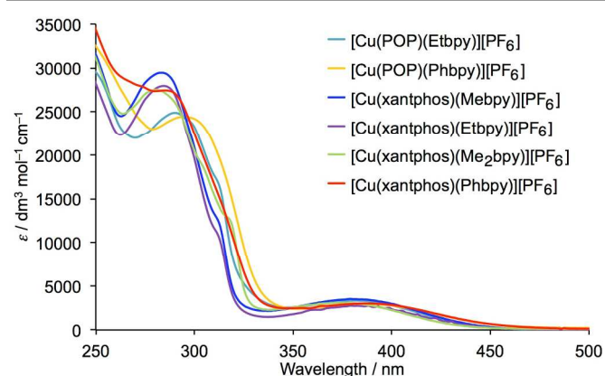
Fig. 7. Solution absorption spectra of the [\text{Cu}(\text{P}^\wedge\text{P})(\text{N}^\wedge\text{N})][\text{PF}_6] complexes ( \text{CH}_2\text{Cl}_2 , 2.5 \times 10^{-5} \text{ mol dm}^{-3} ).
