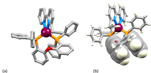
Fig. 5. Structure of the [\text{Cu}(\text{POP})(\text{Etbpy})]^+ cation in [\text{Cu}(\text{POP})(\text{Etbpy})][\text{PF}_6]\cdot\text{Et}_2\text{O} : (a) view of the cation (H atoms omitted for clarity); (b) intra-cation face-to-face \pi -stacking interaction.
