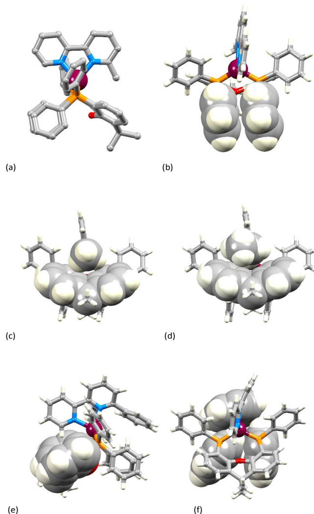
Fig. 3. (a)–(c) The structure of the [\text{Cu}(\text{xantphos})(\text{Mebpy})]^+ cation: (a) view along the P–P vector of the xantphos ligand (H atoms omitted for clarity); (b) face-to-face \pi -stacking of phenyl rings in the two different PPh 2 units; (c) accommodation of the methyl group of Mebpy in the xantphos 'bowl'. (d) A view of the [\text{Cu}(\text{xantphos})(\text{Etbpy})]^+ cation for comparison with the analogous view of [\text{Cu}(\text{xantphos})(\text{Mebpy})]^+ shown in (c). (e)–(f) The structure of the [\text{Cu}(\text{xantphos})(\text{Phbpy})]^+ cation with space-filling representations emphasizing (e) the xanthene 'bowl' with the unsubstituted pyridine ring lying above it, and (f) the phenyl group of Phbpy oriented over two Ph rings of the PPh 2 units.
