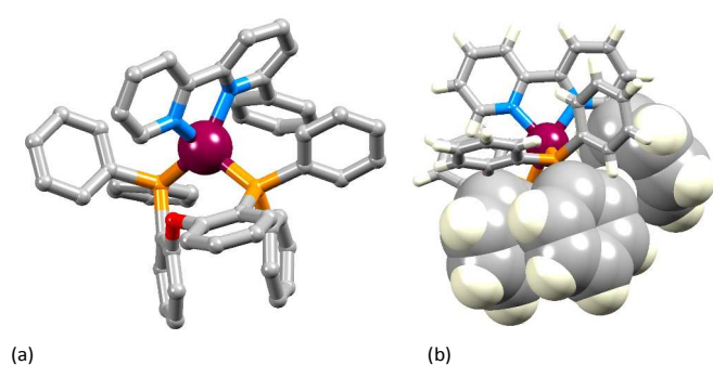
Fig. 6. Structure of the [\text{Cu}(\text{POP})(\text{Ph}bpy)]^+ cation in [\text{Cu}(\text{POP})(\text{Ph}bpy)][\text{PF}_6]\cdot\text{Et}_2\text{O} : (a) view of the cation (H atoms omitted for clarity); (b) intra-cation face-to-face and accompanying edge-to-face \pi -stacking interaction.
