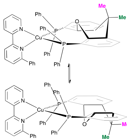
Scheme 4. Proposed conformers of [\text{Cu}(\text{xantphos})(\text{Phbpy})]^+ observed at 205 K in \text{CD}_2\text{Cl}_2 solution, and interconversion pathway through inversion of the xanthene unit. See also Fig. 2.
