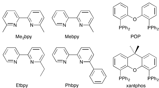
Scheme 2. Atom labelling in [\text{Cu}(\text{POP})(\text{Phbpy})]^+ for NMR spectroscopic assignments. Analogous labelling is used for all [\text{Cu}(\text{P}^{\wedge}\text{P})(\text{N}^{\wedge}\text{N})]^+ complexes.
