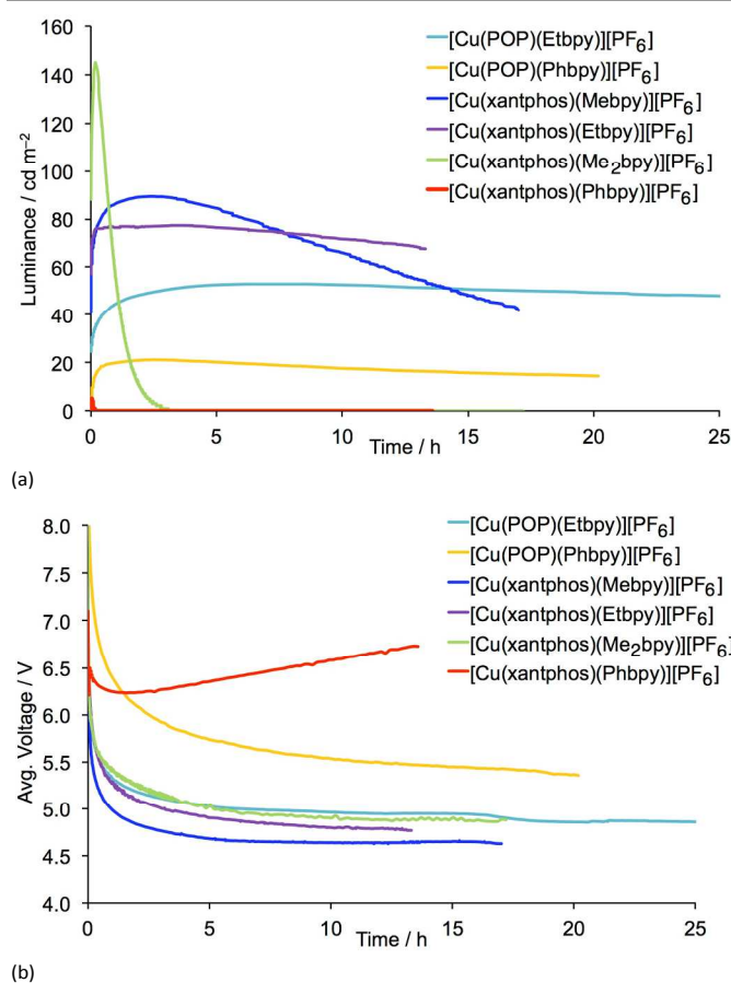
Fig. 10. Luminance (a) and average voltage (b) for ITO/PEDOT:PSS/[Cu(P A )(N A N)][PF 6 ]:[Emim][PF 6 ] 4:1 molar ratio/Al LECs measured using a pulsed current driving (average current density 50 A m -2 , 1
