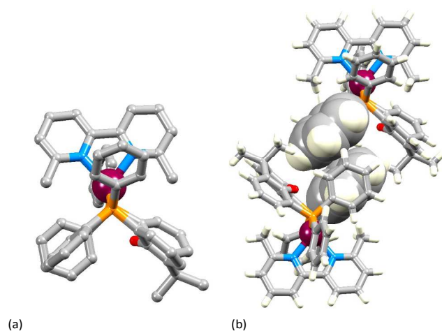
Fig. 4. The structure of the [Cu(xantphos)(Me 2 bpy)] + cation in [Cu(xantphos)(Me 2 bpy)][PF 6 ]: (a) view along the P---P vector of the xantphos ligand (H atoms omitted for clarity); (b) face-to-face π-stacking of PPh 2 phenyl rings between adjacent cations.
