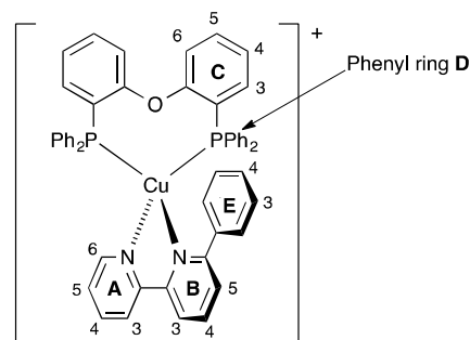
Scheme 2. Atom labelling in [\text{Cu}(\text{POP})(\text{Phbpy})]^+ for NMR spectroscopic assignments. Analogous labelling is used for all [\text{Cu}(\text{P}^{\wedge}\text{P})(\text{N}^{\wedge}\text{N})]^+ complexes.
