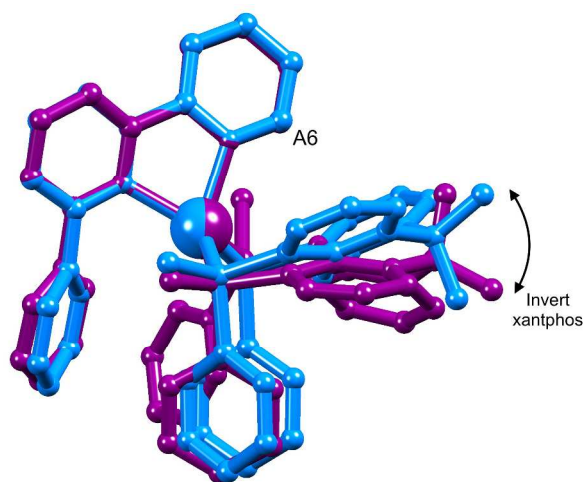
Fig. 2. Overlay of the DFT geometry-optimized structures of two conformers of [\text{Cu}(\text{xantphos})(\text{Phbpy})]^+ which are related by inversion of the xanthene unit (right side of figure); for clarity, H atoms are omitted and only the ipso -C atoms of PPh 2 phenyl rings in front and behind the Cu atoms are shown. The Cu atoms and pairs of corresponding N atoms were overlaid. The position of the bpy H A6 protons is marked as "A6".
