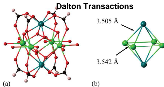
Figure 13. (a) Representation of the Zr_6 cluster geometry found in the zirconium formate compound Zr_6O_4(OH)_4(HCOO)_8 . 61 The equatorial oxygen atoms belong to dangling formate anions, and are disordered over closely-related sites. The two crystallographically-distinct Zr atoms are shown in different shades of green. (b) The central Zr_6 octahedron geometry in this cluster, showing the spontaneous symmetry-lowering of Zr...Zr distances.
