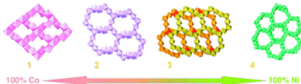
Figure 4. The cobalt/nickel succinates form four different structures with entirely different compositions when crystallized under the same conditions. Reprinted with permission from C. Livage et al, Angew. Chemie Intl. Ed. 46 , 5877 (2007). Copyright 2007. John Wiley and Sons.
