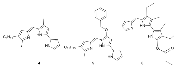
Fig. 3 Examples of B-ring modified prodigiosin analogs.
