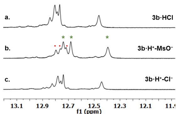
Fig. 4 1 H NMR spectra in CDCl 3 for the pyrrolic NH region of: a) 3b ·HCl; b) after addition of 6 eq of MsOH to sample a, two sets of NH signals were observed for each \alpha (•) and \beta (*) conformer; c) after addition of 1 eq of tetrabutylammonium chloride (TBACl) to sample b.
