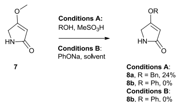
Scheme 1 Direct substitution of pyrrolinone 7 .
