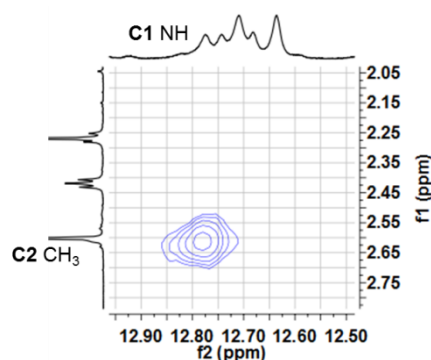
Fig. 5 A region of the 1 H- 1 H NOESY spectrum of 3b ·OMs in CDCl 3 shows a NOE correlation between one of the “minor” pyrrole NH protons and C2 methyl hydrogens. This correlation is consistent with the pyrrolic NH of the C-ring being involved in an intramolecular H-bond with the -OPh group of the B-ring (see Scheme 4).
