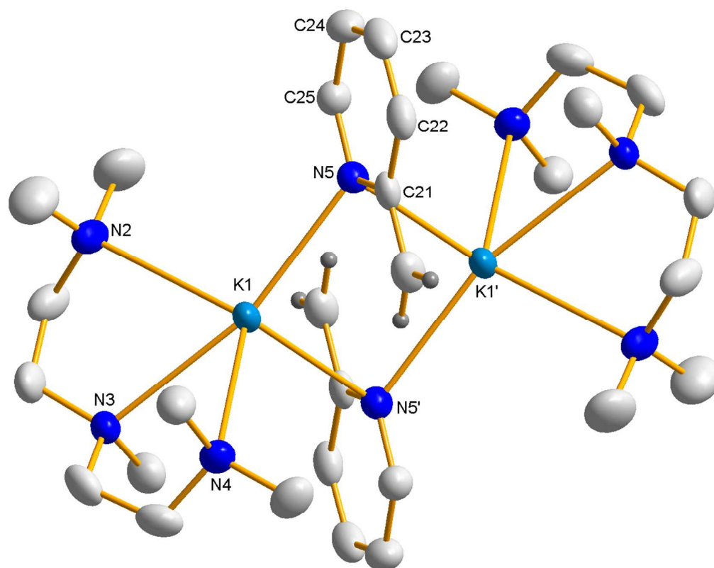
Figure 8 Molecular structure of [2\text{-picK}\cdot\text{PMDETA}]_2 ( 6' ). Ellipsoids are displayed at 50% probability and all hydrogen atoms (except those of the metalated \text{CH}_2 group) and minor disordered component at one end of PMDETA molecule are omitted for clarity. Symmetry operation to generate equivalent atoms labeled ' : 1-x, -y, 1-z . Selected bond lengths ( \text{\AA} ) and angles ( ^\circ ): K1-N2, 2.915(2); K1-N3, 2.857(2); K1-N4, 2.899(2); K1-N5, 2.786(1); K1-N5', 2.815(1); N2-K1-N3, 63.31(4); N2-K1-N4, 113.02(5); N2-K1-N5, 101.80(4); N2-K1-N5', 132.00(5); N3-K1-N4, 62.25(5); N3-K1-N5, 165.03(4); N3-K1-N5', 100.88(5); N4-K1-N5, 127.30(5); N4-K1-N5', 94.04(5); N5-K1-N5', 90.36(5); K1-N5-K1', 89.64(5).
