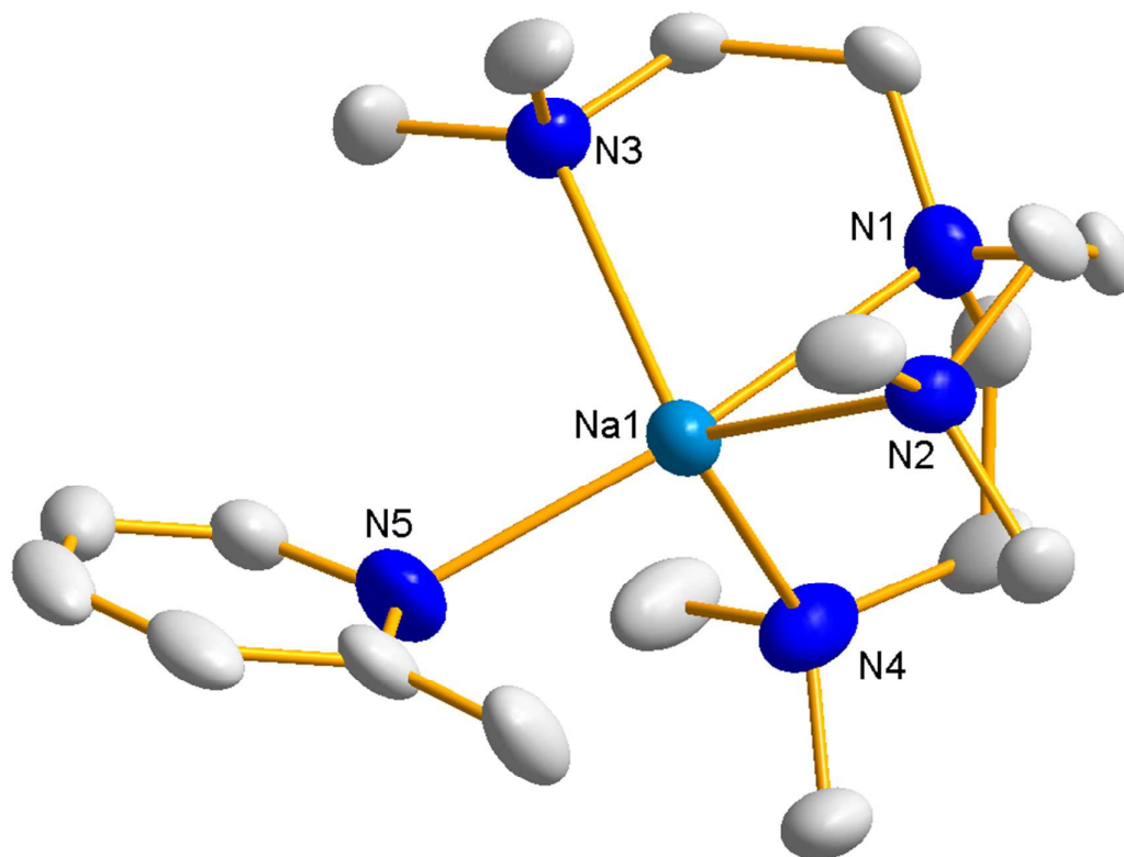
Figure 7 Molecular structure of 2-picNa•Me 6 TREN (5). Ellipsoids are displayed at 50% probability and all hydrogen atoms and minor disordered component of 2-picoyl anion are omitted for clarity.
