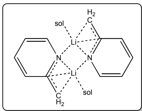
Figure 3 Representation of 2-picolyl lithium molecular structures as revealed by Stalke and co-workers. Sol = \text{OEt}_2 , 2-picH.
