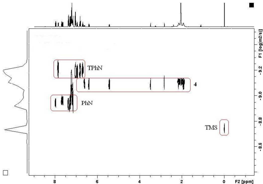
Figure 9 1 H DOSY NMR spectrum of complex 4 in C 6 D 6 solution at 300 K in the presence of inert standards 1,2,3,4-tetraphenyl-naphthalene (TPhN), 1-phenylnaphthalene (PhN) and tetramethylsilane (TMS).
