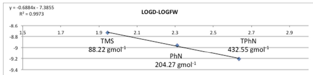
Graph 1 Plot of logD versus logFW from 1 H DOSY NMR data of the mixture of 4 and inert standards TPhN, PhN and TMS in C 6 D 6 solution at 300K
