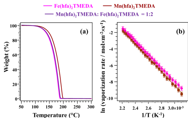
Fig. 1 (a) TGA curves in \text{N}_2 for Mn(hfa) 2 TMEDA (brown), Fe(hfa) 2 TMEDA (pink) and their 1 : 2 mixture (violet). (b) Arrhenius plots for the vaporization of the two precursors (temperature interval \approx 50 \div 180 °C).
