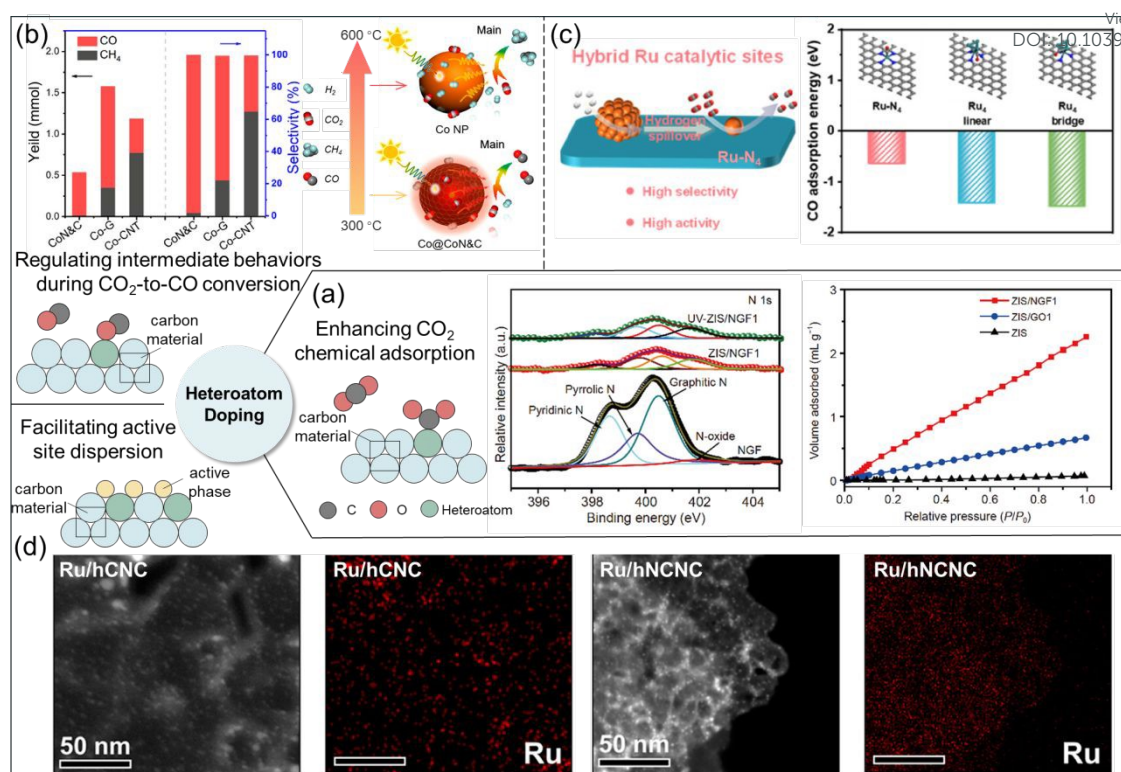
Fig.8 Heteroatom doping in photothermal \text{CO}_2 reduction over carbon materials. (a) Heteroatom doping for enhancing \text{CO}_2 chemical adsorption. Reproduced with permission. 128 Copyright 2020, Science China Press and Springer-Verlag GmbH Germany. Heteroatom doping for regulating intermediate behaviours during the conversion from \text{CO}_2 to CO over (b) \text{Co@CoN\&C} and (c) \text{Ru/hNCNC} . Reproduced with permission. 27 Copyright 2020 American Chemical Society. Reproduced with permission. 112 Copyright 2025, John Wiley & Sons. (d) Heteroatom doping for facilitating active site dispersion. Reproduced with permission. 35 Copyright 2024, American Chemical Society.
