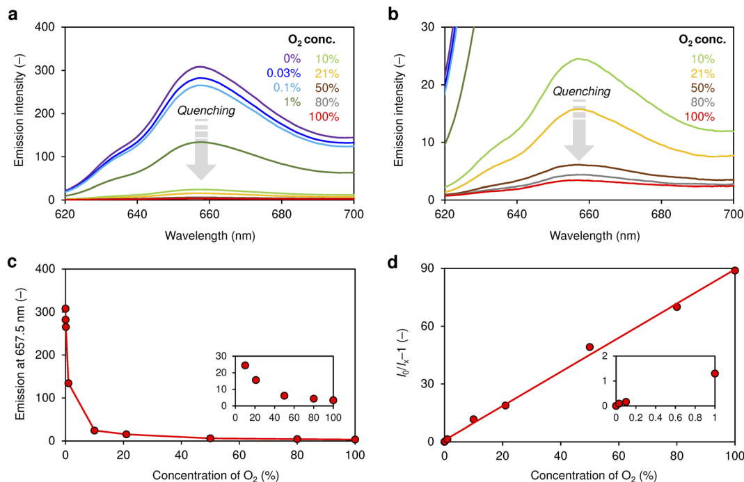
Fig. 3 (a and b) Emission spectra of a neat film PtPL ( \lambda_{\text{ex}} = 412 \text{ nm} ) measured under various O 2 concentrations (a; with higher emission intensities, b; emission intensities lower than 30). See Fig. S10 for photographs illustrating the emission changes of neat PtPL films at different O 2 levels. (c) Plot of O 2 concentration vs. emission intensity ( \lambda_{\text{em}} = 657.5 \text{ nm} ) in a neat film PtPL. Inset shows intensities lower than 30. (d) Stern-Volmer plot of a neat film PtPL ( \lambda_{\text{em}} = 657.5 \text{ nm} ) for O 2 sensing. Inset shows the plot for lower O 2 concentration than 1%. It is worth noting that the phosphorescence of PtPL shows little sensitivity to humidity, whereas it is sensitive to temperature and air pressure (see Fig. S15–17).
