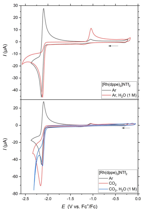
Fig. 5 Cyclic voltammograms of [\text{Rh}(\text{dppe})_2]\text{NTf}_2 . Conditions: 1\text{ mM} \text{Rh}^{\text{I}} in \text{MeCN} , 0.2\text{ M} n\text{Bu}_4\text{NPF}_6 , glassy carbon working electrode, 100\text{ mV s}^{-1} .
