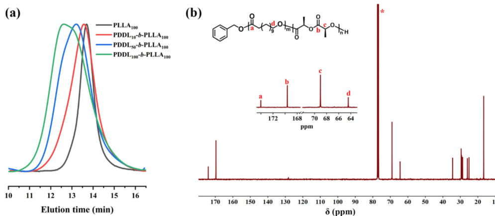
Fig. 3 (a) GPC curves of PLLA (Table 2, run 1) and diblock copolyesters (Table 2, runs 3–5). (b) 13 C NMR spectrum of the block copolyester PDDL- b -PLLA (Table 2, run 4), solvent: CDCl 3 .
