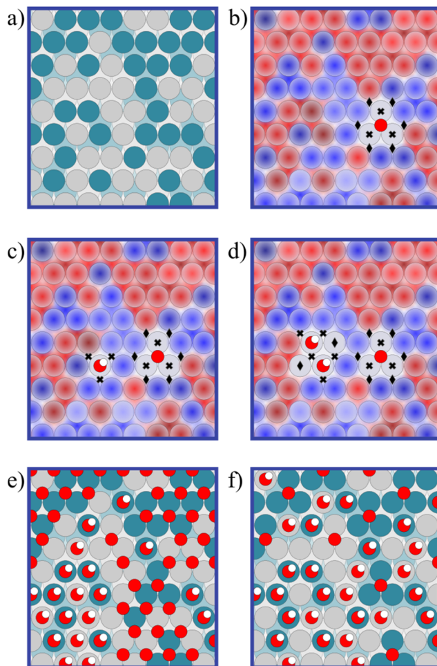
Fig. 3 Illustration of how to fill the solid solution surface shown in (a) using blocking rules. (b) The most stable species (an O^* ) is placed first and blocks three on-top ^*OH sites in mutual blocking (marked by crosses) and an additional six FCC hollow sites in extended blocking (marked by diamonds). (c) The next most stable species (an ^*OH that has not been blocked) in turn blocks three FCC hollow sites (marked by crosses) in both set of rules. (d) The next most stable species (another ^*OH ) blocks additional FCC hollow sites in both set of rules, while the combination of two adjacent ^*OH species blocks the two shared on-top neighbour sites in extended blocking. This process continues until there are no unblocked sites left, resulting in the coverage (e) for mutual blocking and (f) for extended blocking. The colour scheme overlaid in (b)–(d) depicts the GNN-predicted adsorption energy of each site, with the dark red regions indicating strong binding sites (more negative adsorption energy) and the blue regions indicating weak binding sites (more positive adsorption energy).
