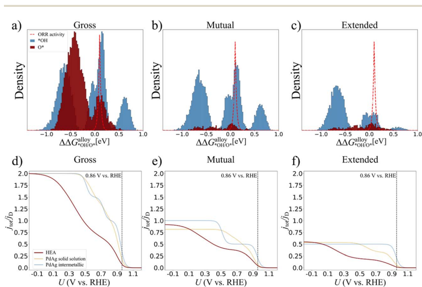
Fig. 7 \text{Ag}_{14}\text{Ir}_{16}\text{Pd}_{30}\text{Pt}_{14}\text{Ru}_{26} HEA (111) surface (a) gross ^*\text{OH}/\text{O}^* adsorption energy distributions and net ^*\text{OH}/\text{O}^* adsorption energy distributions obtained with (b) mutual blocking or (c) extended blocking rules. Potential-dependent ORR current of the PdAg intermetallic, the equimolar PdAg solid solution, and the \text{Ag}_{14}\text{Ir}_{16}\text{Pd}_{30}\text{Pt}_{14}\text{Ru}_{26} HEA given that either (d) the gross distributions, (e) mutual blocking net distributions, or (f) extended blocking net distributions determine the ORR activity.
