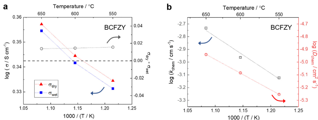
Fig. 4 (a) Electrical conductivity of BCFZY under dry and 3% H 2 O-humidified atmosphere ( p\text{O}_2 = 0.156 atm) at various temperatures. The conductivity decreases under humidified conditions, providing the evidence of hydrogenation behavior. (b) Surface exchange coefficient ( k_{\text{chem}} ) and chemical diffusion coefficient ( D_{\text{chem}} ) of BCFZY as a function of temperature, extracted by fitting ECR data obtained during dehydrogenation.
