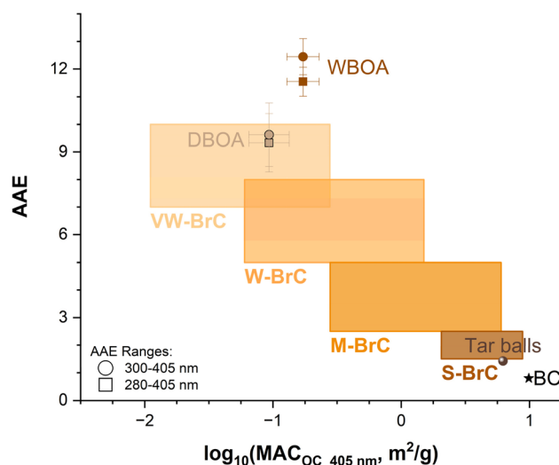
Fig. 3 Classification of WBOA and DBOA mixtures according to the optical framework of Saleh 2020. 4 Average AAE and \log_{10}(\text{MAC}_{\text{OC}_{405 \text{ nm}}}) are calculated for the DBOA and WBOA samples. 44 AAE values are calculated over 280–405 nm (squares) and 300–405 nm (circles) spectral ranges. Reference values for \text{BC}^{76} and strongly absorbing \text{BrC}^{77} are included for visual comparison.
