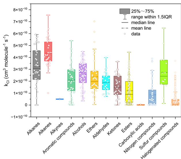
Fig. 1 Rate constants for reactions of Cl atoms with organic compounds. Data from the database for the kinetics of the gas-phase atmospheric reactions of organic compounds. 87,88
