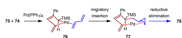
Scheme 20 \text{Pd}(\text{PPh}_3)_4 -catalyzed intermolecular [4+2] cycloadditions of vinylallenes and 1,3-dienes.
