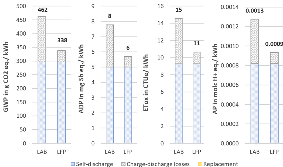
Fig. 4 Impacts of the use phase of the UPS use case on global warming potential (GWP), mineral, fossil & renewable resource depletion (ADP), freshwater ecotoxicity (ETox) and acidification potential (AP). Values are given per kW h of energy delivered over lifetime (FU).
