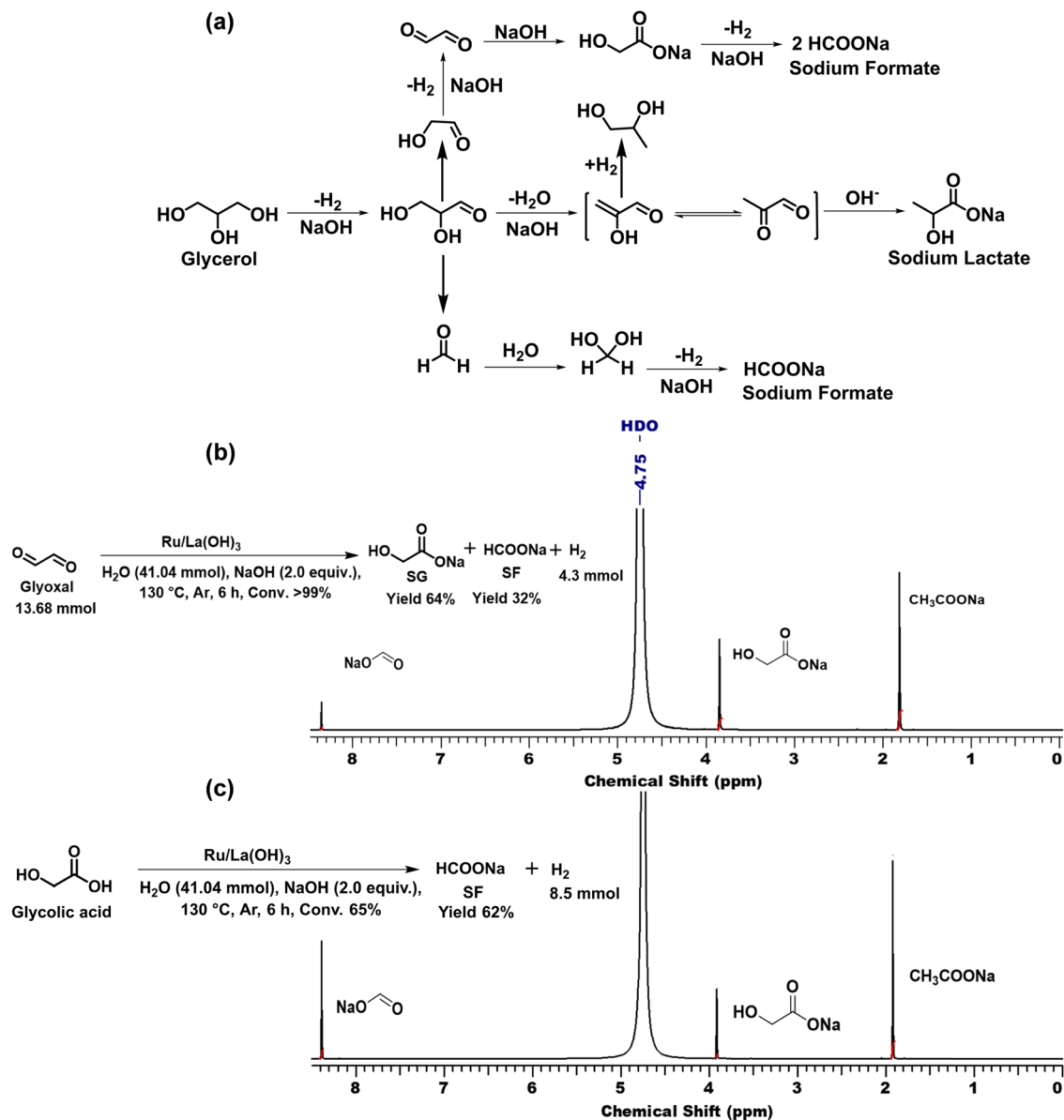
Scheme 1 (a) Plausible reaction pathways for hydrogen production from glycerol over the \text{Ru/La(OH)}_3 catalyst. (b) Control experiment for the transformation of glyoxal over the \text{Ru/La(OH)}_3 catalyst. (c) Control experiment for the transformation of glycolic acid over the \text{Ru/La(OH)}_3 catalyst. Reaction conditions: \text{Ru/La(OH)}_3 (100 mg, 9 wt% Ru), glyoxal/glycolic acid (13.68 mmol), NaOH (27.36 mmol), water (41.04 mmol), 130^\circ\text{C} , and 600 rpm.
