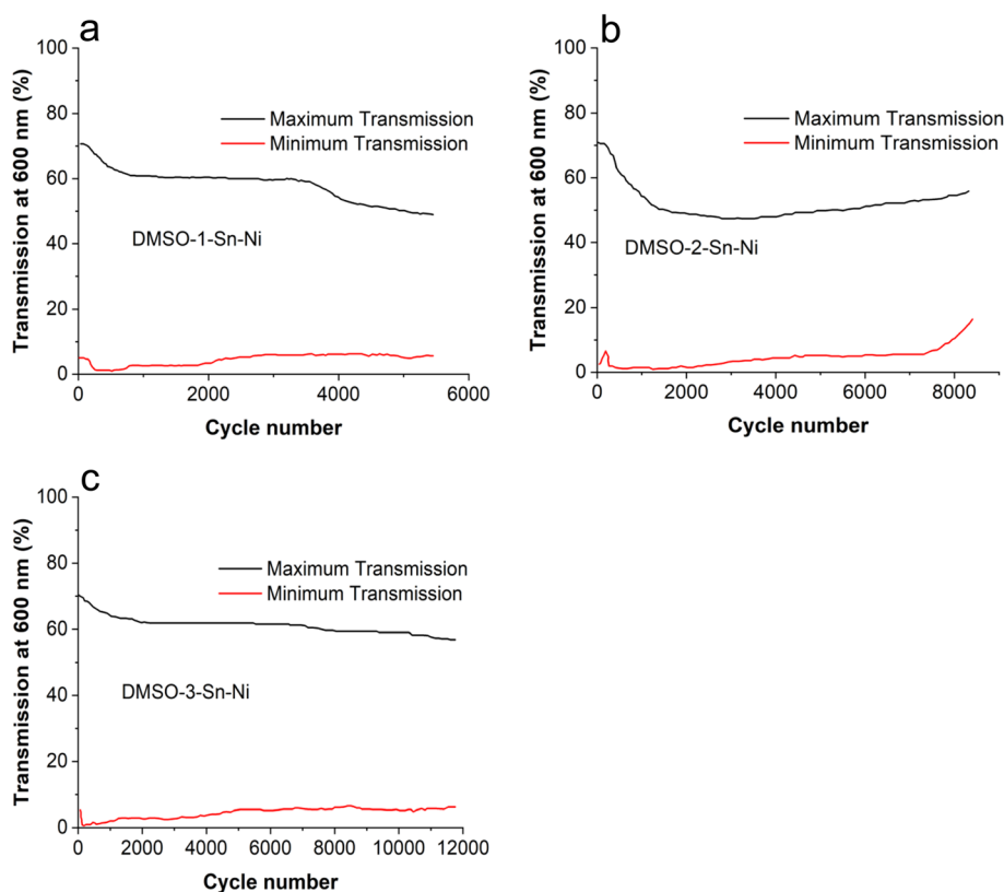
Fig. 7 Minimum and maximum transmission at 600 nm of 25 cm 2 dynamic windows during cycling using various Zn DMSO electrolytes. The windows contain \text{NiCl}_2 , \text{SnCl}_2 , and 5 wt% PVA with the DMSO-1 (a), DMSO-2 (b), and DMSO-3 (c) formulations. In all cases, each switch cycle consisted of -0.8 V for 30 s to induce device darkening followed by +1.0 V for 60 s to induce device lightening.
