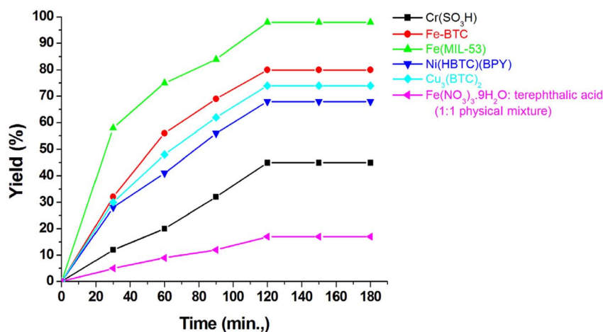
Fig. 4 Optimisation of different MOFs as catalysts for the synthesis of xanthenone (4a). a Reaction conditions: catalyst (20 wt%), benzaldehyde (0.71 mmol, 1.0 eq.), dimesone (1.42 mmol, 2.0 eq.), ethanol (2.0 mL), reflux. Reaction monitored by HPLC.
