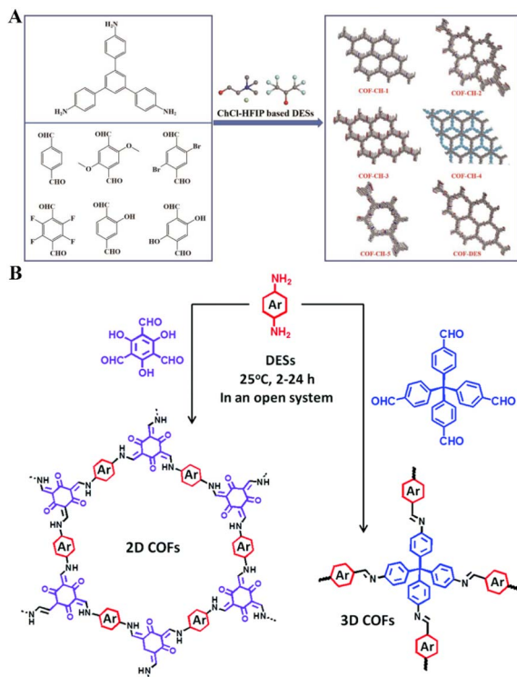
Fig. 6 Framework materials fabrication via precipitation, utilizing DES as the reaction medium. (A) Preparation processes of the selected imine-linked COFs. Reprinted with permission from copyright© American Chemical Society, 2023. 92 (B) Schematic illustration of the syntheses of 2D and 3D COFs. Reprinted with permission from copyright© Royal Society of Chemistry, 2020. 95
