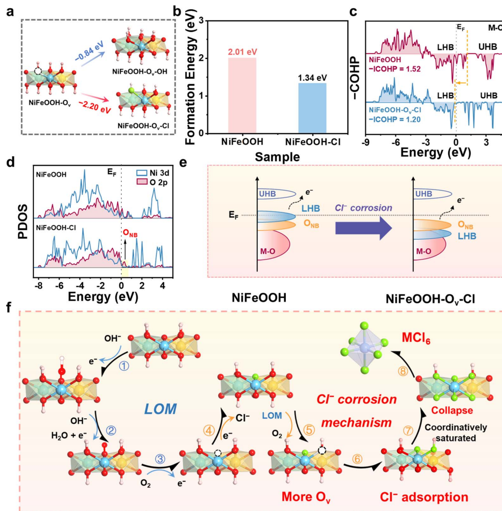
Fig. 4 Elucidation of the corrosion mechanism of NiFe LDH. (a) Comparison of the calculated adsorption energies of \text{Cl}^- and \text{OH}^- on the \text{O}_\text{v} of NiFeOOH; (b) calculated formation energy of \text{O}_\text{v} ; (c) -\text{COHP} analysis; (d) PDOS of NiFeOOH and NiFeOOH- \text{Cl} ; (e) schematic energy bands of NiFeOOH and NiFeOOH- \text{O}_\text{v} - \text{Cl} ; (f) comprehensive schematic illustrating the self-reinforcing corrosion cycle perpetuated by the preferential adsorption of \text{Cl}^- , which ultimately leads to the rapid degradation of the NiFe LDH structure.
