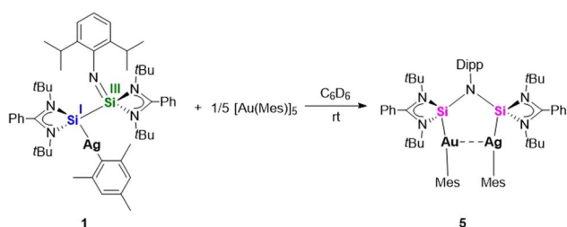
Scheme 4 Synthesis of the heterobimetallic bis-silylene complex [ \text{LSi}\{\text{Ag}(\text{Mes})\}(\text{NDipp})\text{-}\{\text{Au}(\text{Mes})\}\text{SiL} ] (5).
