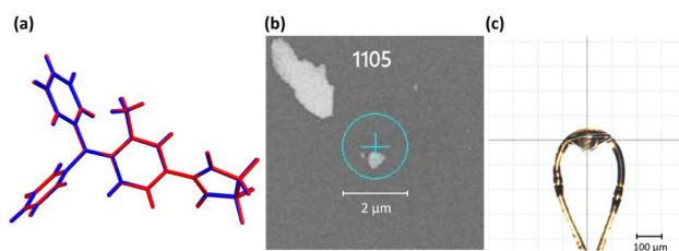
Fig. 6 (a) Electron diffraction and SC-XRD structure overlay for 3a – ED (red) and SC-XRD (blue); (b) visual image of representative grain used for ED data collection; (c) visual image of crystal used for SC-XRD. Note the scale bars.
