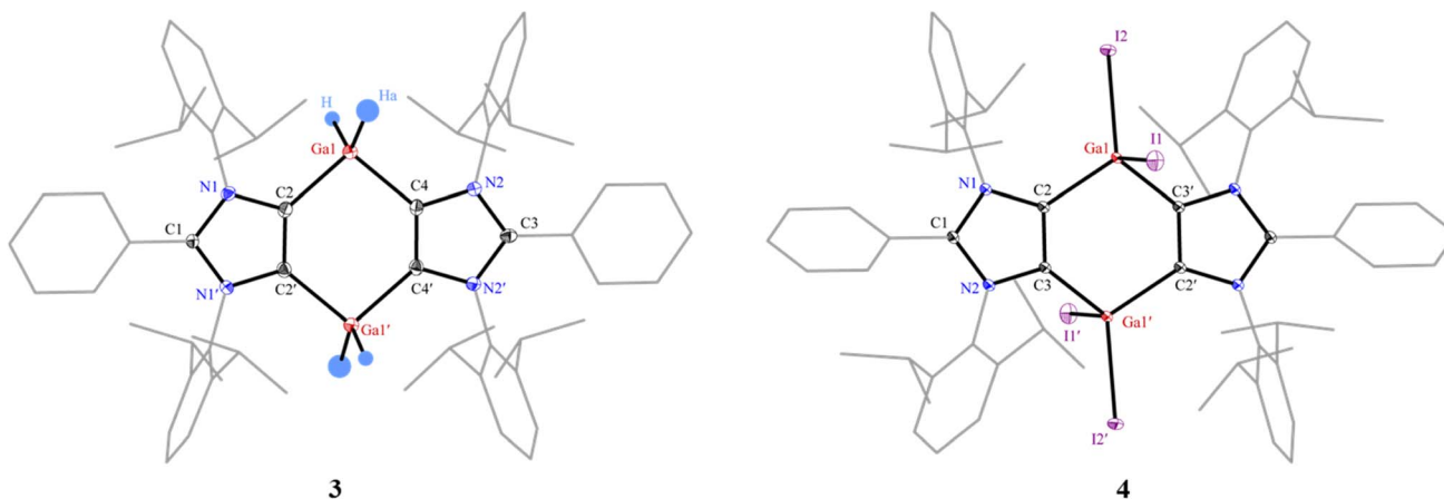
Fig. 2 Solid-state molecular structures of 3 and 4. Hydrogen atoms (except on \text{GaH}_2 for 3) and two benzene molecules (for 3) are omitted for clarity. Aryl groups are depicted as wireframes. Thermal displacement ellipsoids at 50%. Selected bond lengths (Å) and angles ( ^\circ ) for 3: C2–Ga1 2.016(3), C4–Ga1 2.015(3), C2'–C2 1.377(6), C2–Ga1–C4 101.2(1), symmetry code: 2 - x, 1 - y, z ; and for 4: C2–Ga1 1.993(1), C3'–Ga1 1.993(1), Ga1–I1 2.6117(1), Ga1–I2 2.5230(1), C2–C3 1.378(1), I1–Ga1–I2 107.47(1), C2–Ga1–I1 100.14(2), C2–Ga1–I2 117.85(2), C2–Ga1–C3' 107.36(3), symmetry code: 1 - x, 1 - y, 1 - z .
