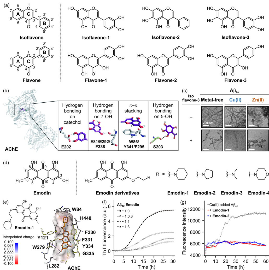
Fig. 8 Examples of chemical reagents regulating metal-free or metal-bound Aβ and AChE. (a) Structures of flavonoids. Isoflavone , 3-phenyl-4H-chromen-4-one; isoflavone-1 , 3-(3,4-dihydroxyphenyl)-5,7-dihydroxy-4H-chromen-4-one; isoflavone-2 , 5,6,7-trihydroxy-3-phenyl-4H-chromen-4-one; isoflavone-3 , 2-phenyl-4H-chromen-4-one; flavone , 2-(3,4-dihydroxyphenyl)-3,5,7-trihydroxy-4H-chromen-4-one; flavone-1 , 2-(3,4-dihydroxyphenyl)-3,5,7-trihydroxy-4H-chromen-4-one; flavone-2 , 2-(3,4-dihydroxyphenyl)-5,7-dihydroxy-4H-chromen-4-one; flavone-3 , 2-(4-hydroxyphenyl)-3,5,7-trihydroxy-4H-chromen-4-one. (b) Intermolecular interactions between the flavonoids and AChE. Reproduced with permission from ref. 289 and 292. Copyright© 2023 Royal Society of Chemistry and 2020 Royal Society of Chemistry. (c) Impact of isoflavone-3 on the formation of metal-free Aβ 42 and metal-Aβ 42 aggregates. The morphology of the resultant Aβ 42 species was analyzed by TEM. Reproduced with permission from ref. 289. Copyright© 2023 Royal Society of Chemistry. (d) Structures of emodin and its derivatives with different functional groups at the R position. Emodin , 1,3,8-trihydroxy-6-methylanthracene-9,10-dione; emodin-1 , 1,8-dihydroxy-3-methyl-6-(2-(piperidin-1-yl)ethoxy)anthracene-9,10-dione; emodin-2 , 1,8-dihydroxy-3-methyl-6-(2-(pyrrolidin-1-yl)ethoxy)anthracene-9,10-dione; emodin-3 , 1,8-dihydroxy-3-methyl-6-(2-(dimethylamino)ethoxy)anthracene-9,10-dione; emodin-4 , 1,8-dihydroxy-3-methyl-6-(2-morpholinoethoxy)anthracene-9,10-dione. (e) Binding of emodin-1 against AChE. Reproduced with permission from ref. 291. Copyright© 2024 Elsevier. (f) Effect of emodin on Aβ 42 aggregation. The inhibitory activity of emodin on the production of β-sheet-rich Aβ 42 aggregates was quantitatively measured by the ThT assay. Reproduced with permission from ref. 101. Copyright© 2021 John Wiley and Sons. (g) Impact of emodin-1 and emodin-2 on Cu(II)-induced Aβ 42 aggregation. The influence of emodin-1 and emodin-2 on the generation of β-sheet-rich Cu(II)-Aβ 42 aggregates was analyzed by the ThT assay. Reproduced with permission from ref. 293. Copyright© 2023 Springer Nature.
