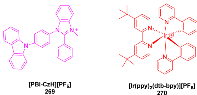
Fig. 112 Chemical structure of first-generation carbazole (Cz)-based ionic host material (270). 332
