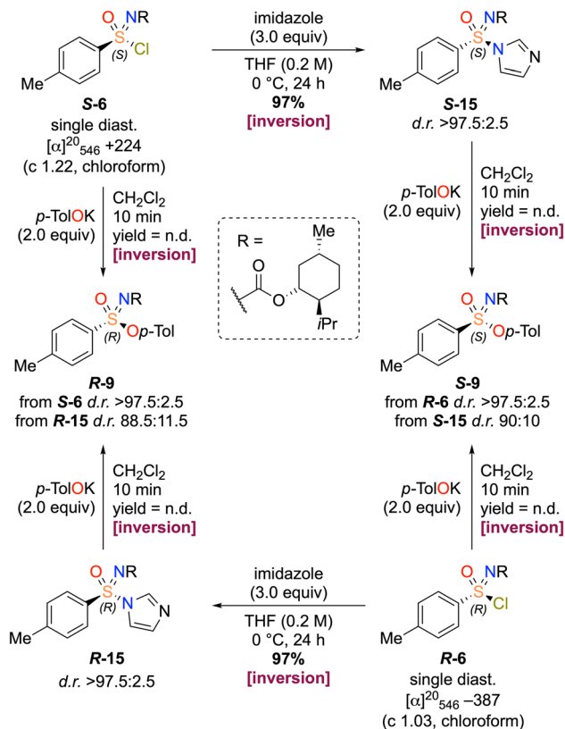
Scheme 3 Route to synthesise sulfonimidates R-9 and S-9 from sulfonyl chlorides S-6 and R-6 and sulfonimidoyl imidazoles R-15 and S-15 , with all steps proceeding with inversion of stereochemistry. n.d. = not determined.
