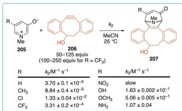
Fig. 30 Kinetic study of the (5 + 2) cycloaddition of oxido-3-pyridinium betaines with 4-dibenzocyclooctynol.
