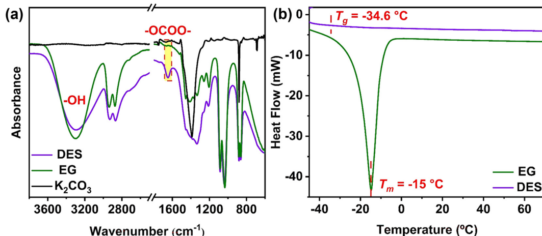
Fig. 2 FT-TR spectra (a) and DSC thermograms (b) of the DESs.
