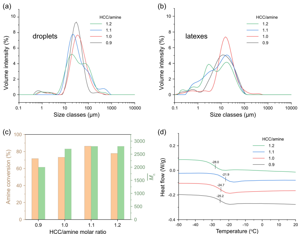
Fig. 6 Effect of the HCC/amine ratio on (a) droplet size distribution, (b) latex size distribution, and (c) amine conversion determined by ^1\text{H} NMR and \overline{M}_n determined using polystyrene standards on SEC, and (d) DSC thermograms from the second heating ramp of WNIPU latexes stabilized with a CNC concentration at an m_p of 8 \text{ mg mL}^{-1} .
