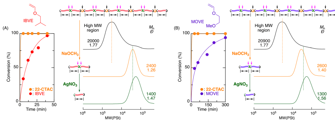
Fig. 8 Cationic DT copolymerization of IBVE (A) and MOVE (B) with 22-CTAC and SEC curves before and after stepwise degradation: [VE]_0/[22-CTAC]_0/[1]_0/[ZnCl_2]_0 = 4000/200/20/4.0 mM in CH_2Cl_2/n -hexane/ Et_2O (20/10/10) at -40 °C. [Thioacetal\ unit]_0/[AgNO_3]_0 = 5.0/50 mM in THF/ H_2O at 20 °C. [Carbonate]_0/[NaOCH_3]_0 = 5.0/50 mM in CH_3OH at 60 °C.
