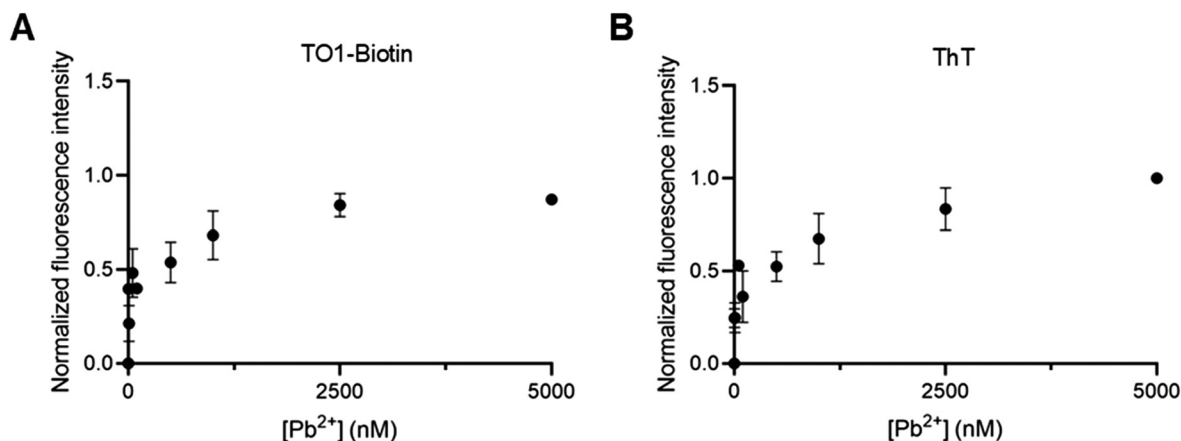
Fig. 6 Mango lead sensors are functional in tap water. Fluorescence signals exhibited by RNA Mango in response to increasing concentrations of \text{Pb}^{2+} in tap water for (A) TO1-biotin and (B) ThT. Experiments were performed at pH 8 and 5 mM \text{Mg}^{2+} . Concentrations of RNA and the dye were 100 nM and 1 \mu\text{M} , respectively, with \text{Pb}^{2+} concentrations in the range of 5 nM–5 \mu\text{M} . Error bars correspond to the standard deviation of three independent experiments.
