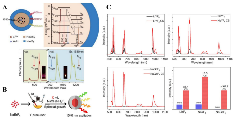
Fig. 2 (A) Energy transfer mechanism in the \text{NaErF}_4 :2% \text{Ho}^{3+} @ \text{NaYF}_4 core/shell UCNPs and the upconversion emission spectrum of the obtained NIR-II UCNPs. 16 (B) Schematic illustration of the synthesis of the series of core-shell upconversion nanoparticles. 17 (C) UC emission spectra of core-shell nanoparticles, and the integration of their emission peaks excited at 1532 nm. 18
