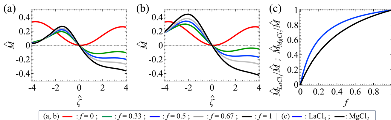
Fig. 5 (a) The non-dimensionalized diffusioophoretic mobility \hat{M} versus the non-dimensionalized colloid surface potential \hat{\zeta} in the same porous media (the ratio of the screening length to the colloid radius l/a = 0.75 ) saturated with solution mixtures of p molar of KCl and q molar of LaCl 3 with different compositions f = q/(p + q) . The solution ionic strength I = 1 mM. Red line: f = 0 . Green line: f = 0.33 . Blue line: f = 0.5 . Grey line: f = 0.67 . Black line: f = 1 . (b) \hat{M} versus \hat{\zeta} in the same porous media ( l/a = 0.75 ) saturated with solution mixtures of p molar of KCl and q molar of MgCl 2 with different compositions f = q/(p + q) . The color scheme and the ionic strength are the same as (a). (c) The ratio of the contribution to the mobility by the asymmetric electrolyte to that by the mixture \hat{M}_{\text{LaCl}_3}/\hat{M} and \hat{M}_{\text{MgCl}_2}/\hat{M} versus f . Blue line: \hat{M}_{\text{LaCl}_3}/\hat{M} . Black line: \hat{M}_{\text{MgCl}_2}/\hat{M} .
