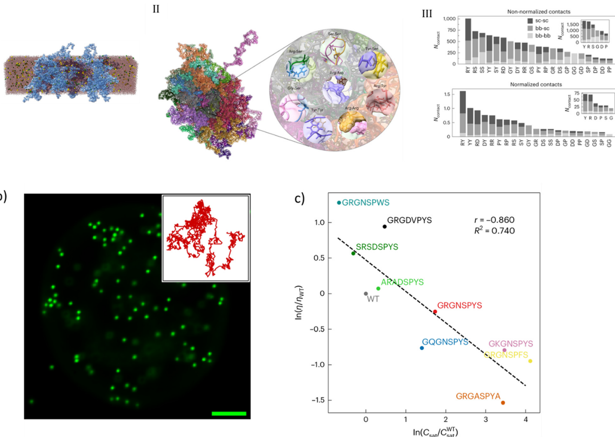
Fig. 3 a) (I): Representative rendering of the atomistic simulation of the condensed phase of [GRGDSPYS] 25 . (II): Snapshot from atomistic simulations of [GRGDSPYS] 25 , highlighting representative examples of the wide variety of contacts driving phase separation of WT. (III): Non normalized (top) and normalized (bottom) average residue pairwise contacts (top), separated into backbone-backbone (bb-bb), backbone-side chain (bb-sc) and side chain-side chain (sc-sc). The inset show the average contacts formed by Tyr:Ser Tyr:Tyr Arg:Asp Arg:Tyr Arg:Arg Arg:Ser. b) Fluorescence microscopy image of 0.5 \mu\text{m} yellow-green fluorescent polystyrene beads embedded in IDP coacervates. Scale bar, 5 \mu\text{m} . Inset: Representative trajectory from two-dimensional particle tracking showing Brownian motion of the beads (the length of the inset box is 0.02 \mu\text{m} ). c) State diagram showing saturation concentration, C_{\text{sat}} , at 18 ^{\circ}\text{C} and viscosities for the variants. Reprinted with permission. 53 Copyright 2024, Springer Nature Limited.
