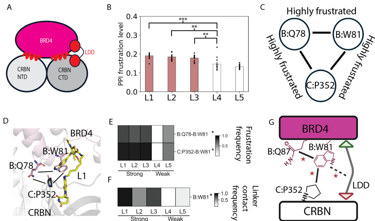
Fig. 2 Frustration in the BRD4-LDD-cereblon complex. In this figure, CRBN stands for cereblon. A) A 2D scheme to show the PPI region (red curve) considered for frustration calculation in this study. B) PPI frustration level comparison among the five LDDs complex. P -Value for significance: L1-L4: 0.0003; L2-L4: 0.001; L3-L4: 0.004. L1-L5: 3.8 \times 10^{-10} ; L2-L5: 4.3 \times 10^{-9} ; L3-L5: 6.9 \times 10^{-8} . C) The top 3 persistent (in terms of frequency in MD simulations) highly frustrated contact pairs in L1 shown as cartoon. D) The top 3 persistent (in terms of frequency in MD simulations) highly frustrated contact pairs in L1 mapped on the 3D structure. The short black lines show the persistent highly frustrated contact pairs. BRD4's cartoon and sidechains are in pink. Cereblon's cartoon and sidechains are in grey. E) Heatmap of frequencies of highly frustrated residue pairs in the BRD4-cereblon interface and between PPI residue pairs. Pairs that are shown here are those with significant difference ( p value < 0.05) between strong and weak LDD system and frequency greater than 70% in at least one system. F) Contact frequency between LDDs' linker and protein residues, with contact frequency greater than 70% in at least one system. B stands for BRD4. G) Proposed mechanism scheme to explain how LDD linker affects PPI frustration. Dashed line refers to LDD linker-protein residue contact. Solid lines refer to protein residue frustration.
