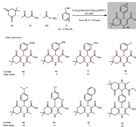
Scheme 46 Catalytic synthesis of hexahydroquinoline derivatives using an Fe 3 O 4 @SiO 2 @Si-(CH 2 ) 2 @HMMA@Cu nanocomposite (Salem et al. ).
