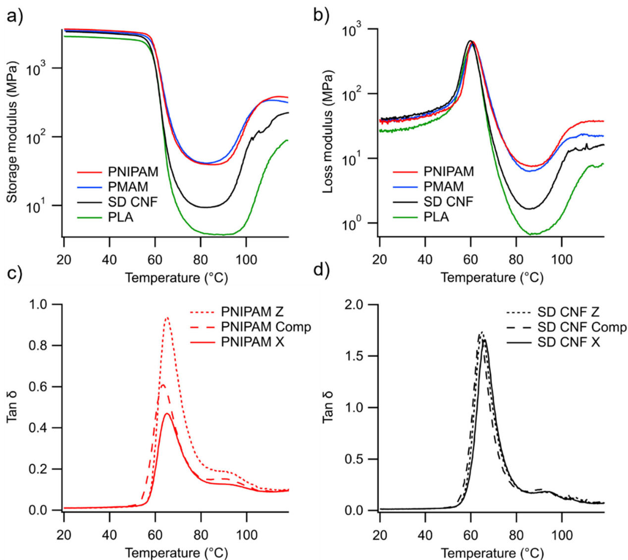
Fig. 8 DMA analysis showing (a) storage moduli and (b) loss moduli of the x-directional samples as a function of temperature. Tan delta of the (c) PNIPAM-MetCNF and (d) SD CNF composites in the x- and z-printing directions as a function of temperature.
