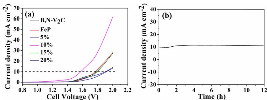
Fig. 9 (a) Polarization curves. (b) Chronoamperometry plot at an applied voltage of 1.57 \text{ V}@j_{10} \text{ mA cm}^{-2} for the 10% \text{FeP@B,N-V}_2\text{C}||10\% \text{ FeP@B,N-V}_2\text{C} as the anode and cathode for overall water splitting in 1 M KOH.
