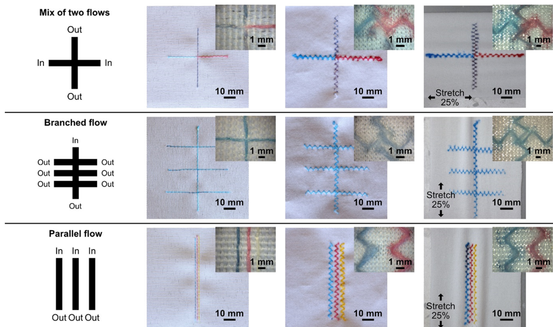
Fig. 2 Fundamental microfluidic functions using stitched Coolmax® threads in hydrophobic fabrics. The leftmost column shows a schematic of each function. The three columns to the right show photographs of the corresponding function realized, in order: in woven, knitted, and stretched knitted fabric. The top corners show the corresponding microscope magnification of the stitches.
