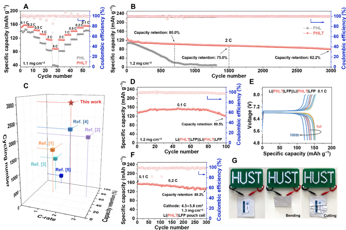
Fig. 6 (A) Rate capabilities and (B) cycling stability of the \text{Li}|\text{PHLT}|\text{LFP} cells. (C) A comparison of C-rate, cycling number, and capacity retention between this work and other reported PVDF-based electrolytes in recent literature. (D) Cycling stability and (E) charge/discharge voltage profiles of the bipolar stacking cell. (F) The cycling performance of a \text{Li}|\text{PHLT}|\text{LFP} pouch cell at 0.2 C. (G) Optical photographs illustrating the bending and cutting tests of the pouch cell.
