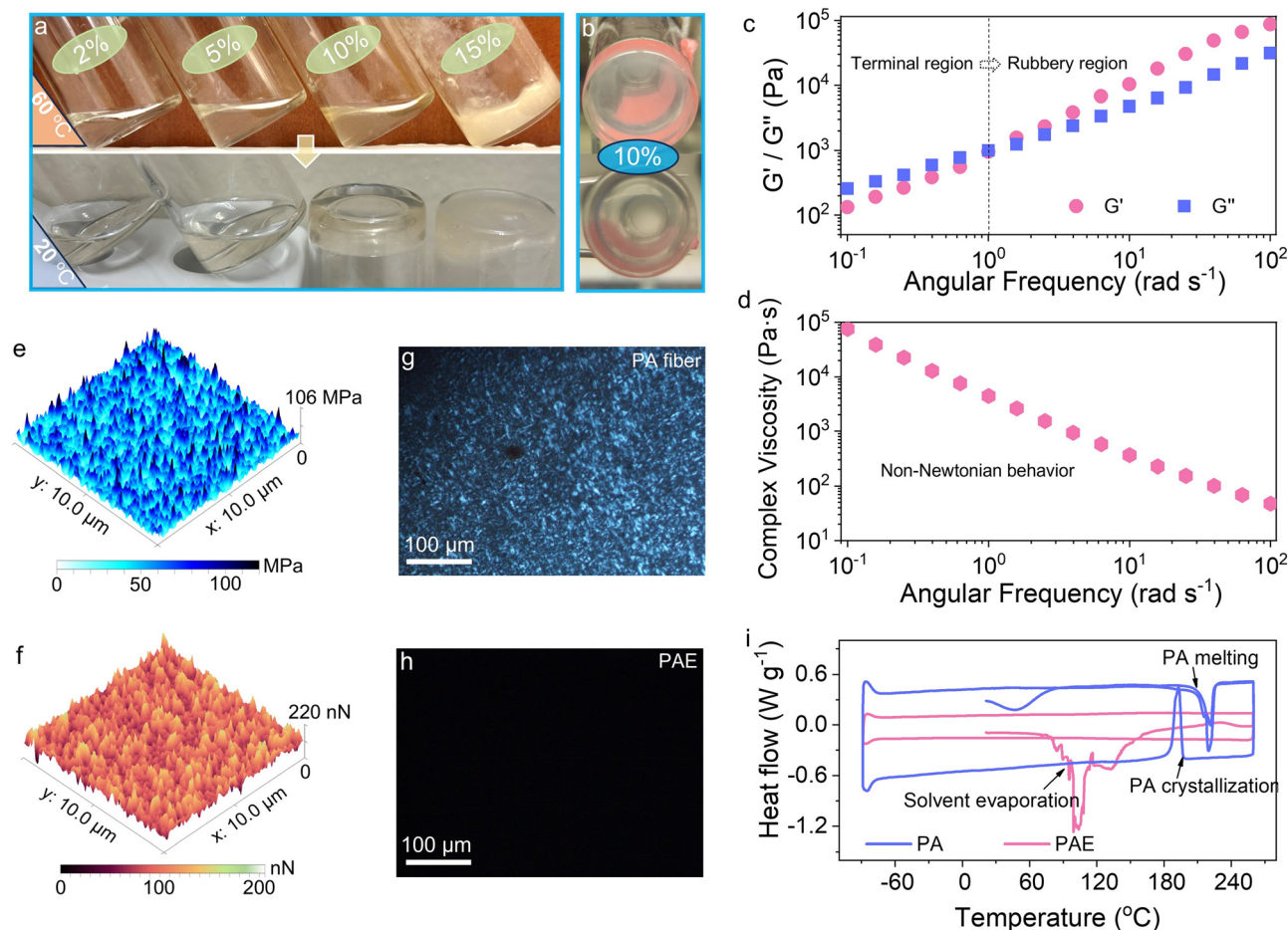
Fig. 2 Nylon electrolyte preparation and mechanical properties. (a) Photographic images illustrating the dissolution of PA in BE at different weight concentrations, observed at 60 °C and 20 °C. (b) Photographic images depicting the dissolution of PA in BE at a weight concentration of 10%. (c) Rheological study of PAE, with G' representing the storage modulus and G'' representing the loss modulus. (d) Plot of complex viscosities of PAE against angular frequency. Measurement of (e) Young's modulus and (f) adhesion force of PAE obtained via atomic force microscopy (AFM). Polarized light microscopy images of (g) PA 6 fiber and (h) PAE. (i) DSC results for PA and PAE over the temperature range of -90 to 260 °C.
