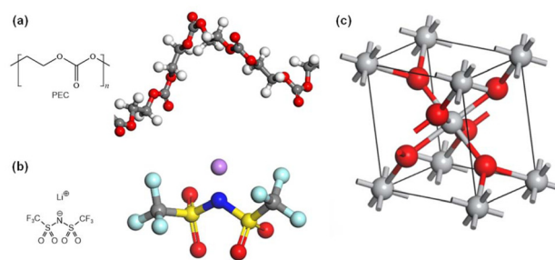
Fig. 1 Chemical structures and molecular models of (a) a PEC chain, (b) LiTFSI and (c) a unit cell of rutile \text{TiO}_2 .
